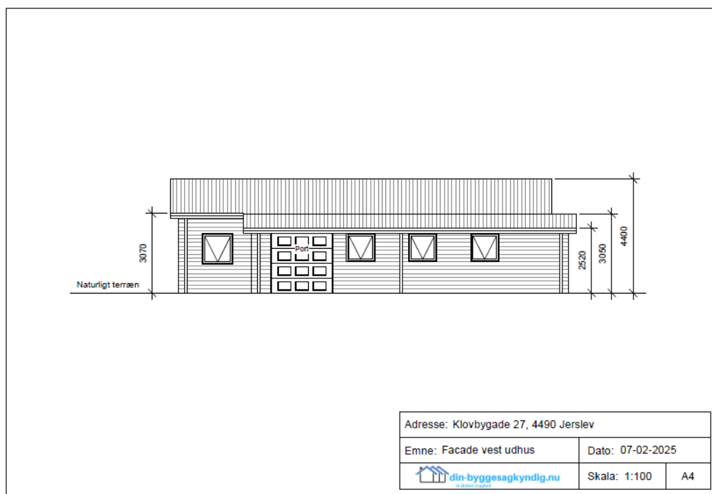
3 – Facadetegning, Vest.
